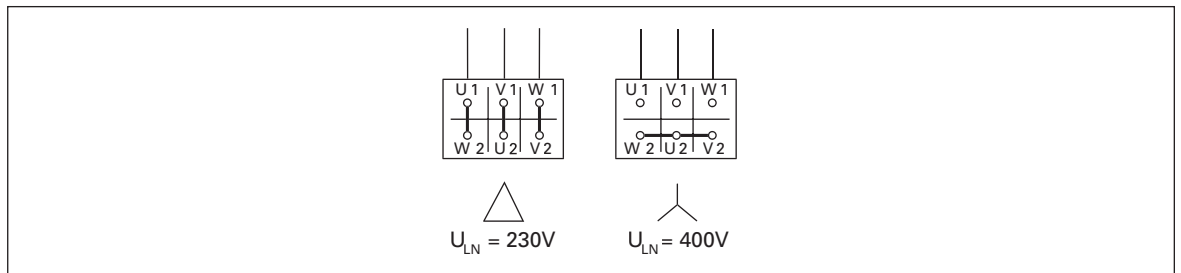
Figure 15: Circuits (Delta, Star)
